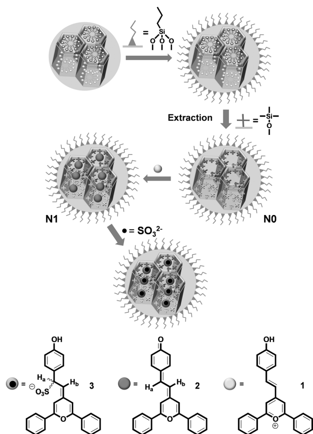
Scheme 1. Representation of the preparation of N0 nanoparticles, the final sensing material N1 (with probe 2 located inside the hydrophobic cavities), and proposed chromofluorogenic reaction with sulfite anion.
